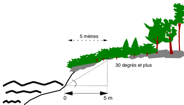
Figure 2.7d : Talus
