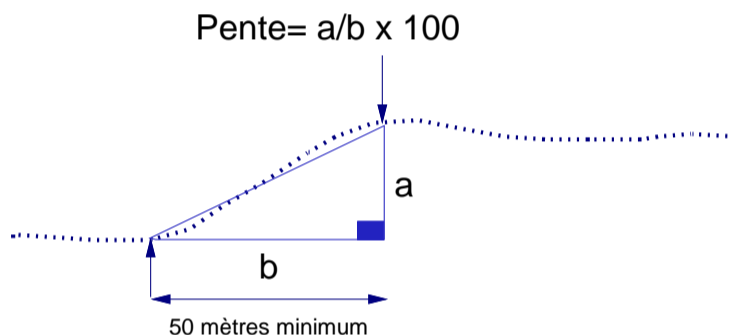
Figure 2.7c : Pente
